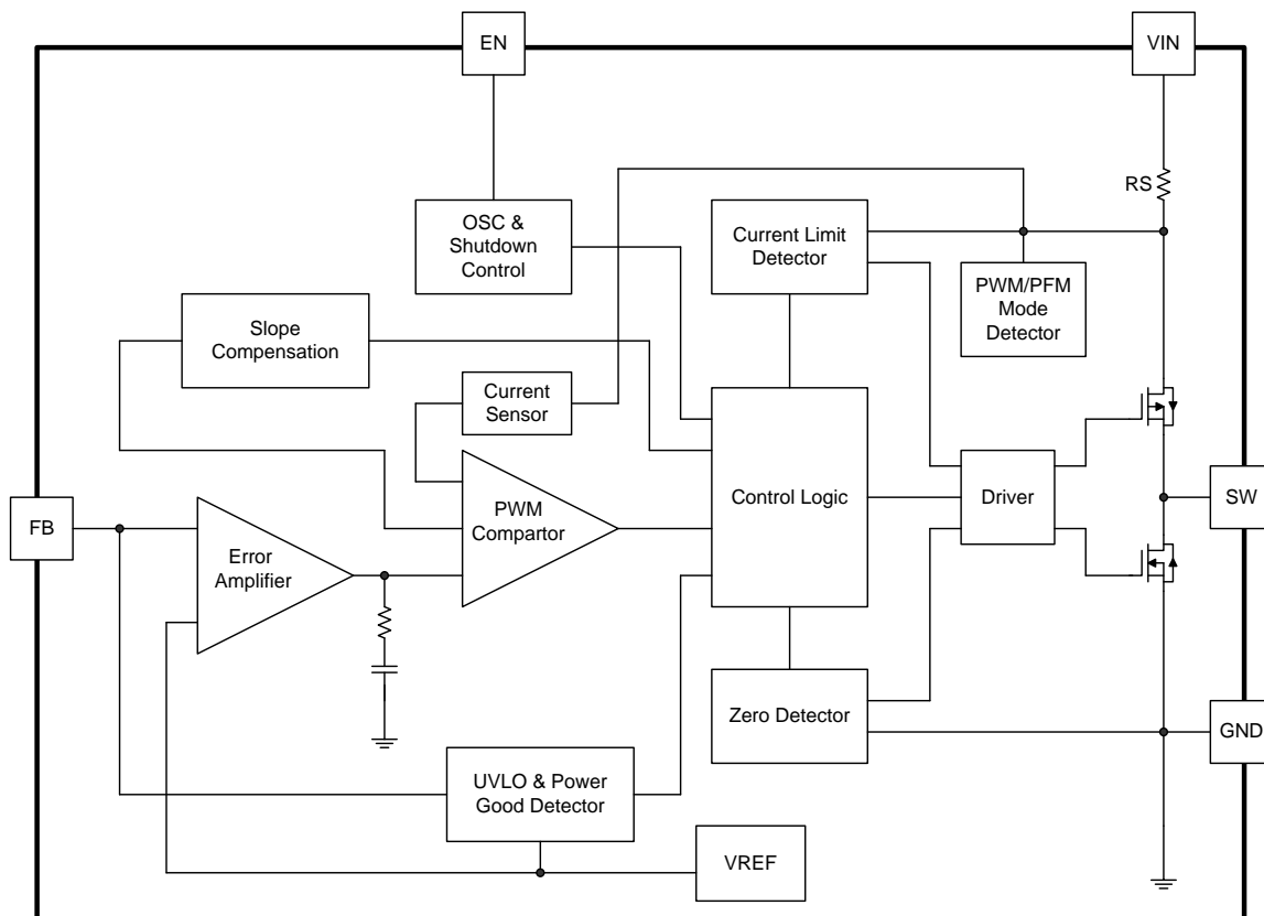
Figure 1. RY3430 Block Diagram
