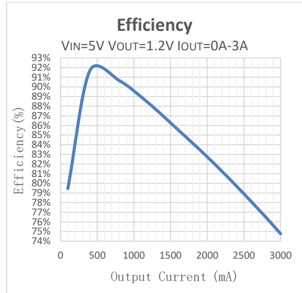
Efficiency V_{OUT}=1.2V
