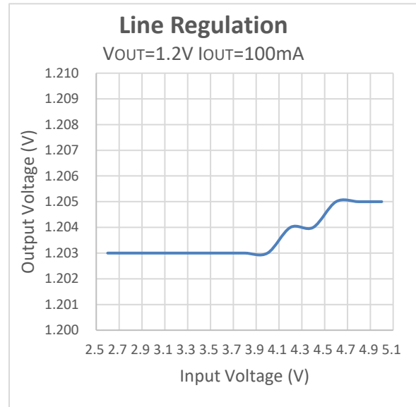
Line Regulation V OUT =1.2V
