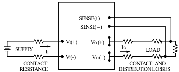
Figure 11. Circuit Configuration for remote sense.
