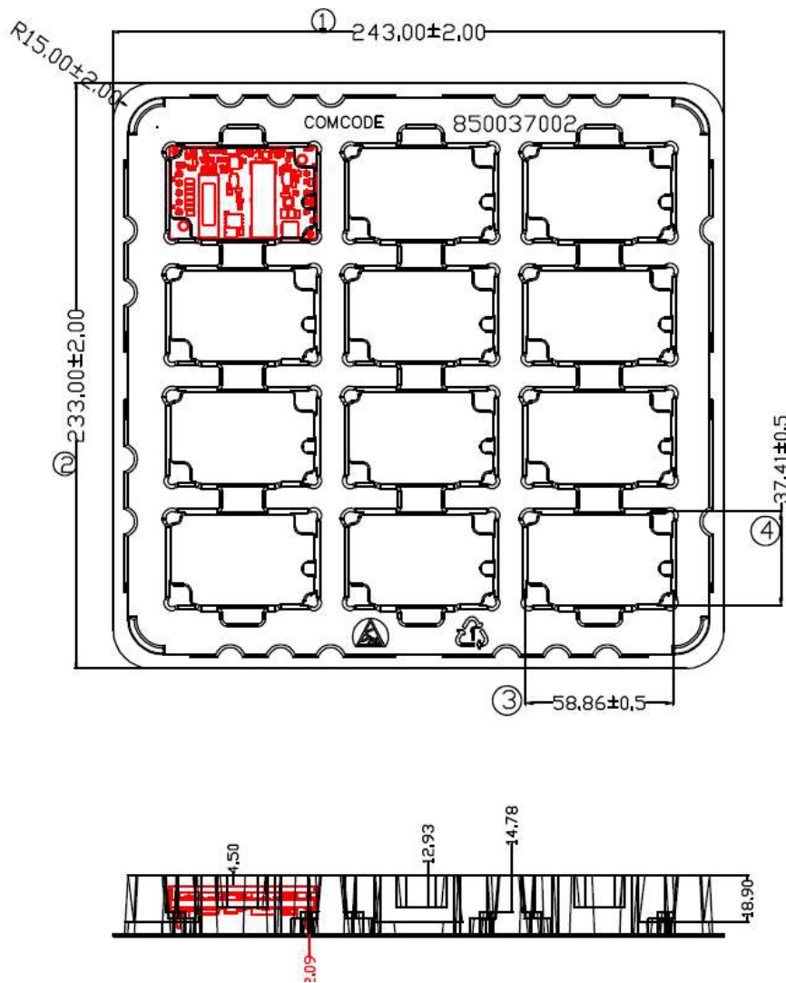
Figure 27. Heat Plate version Packaging Tray
