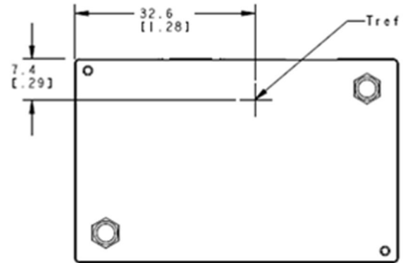
Figure 14. T_{ref} Temperature Measurement Location for heat plate version.
