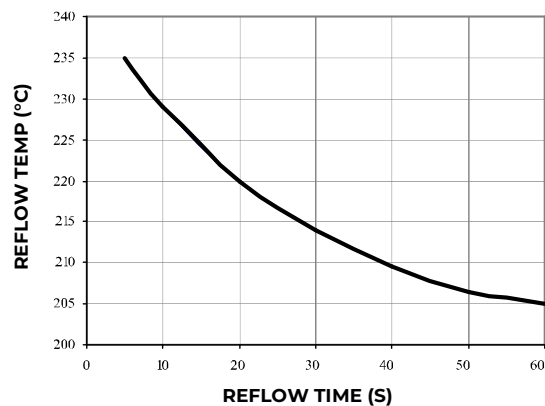
Figure 23. Time Limit Curve Above 205°C for Tin/Lead (Sn/Pb) process
