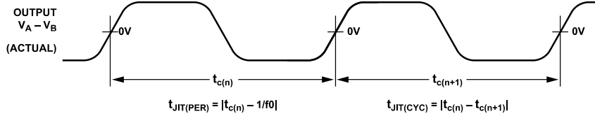
Figure 33. Driver Period, Cycle to Cycle, Random and Deterministic Jitter Characteristics
