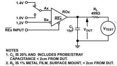
Figure 36. Receiver Enable and Disable Time Circuit
