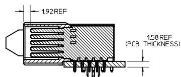
SECTION Z-Z
