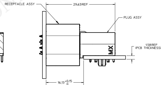
MATED PROFILE
