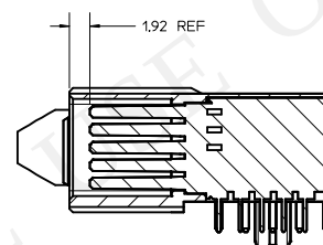
SECTION Z-Z
