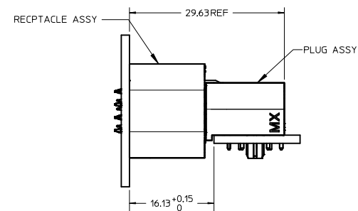
MATED PROFILE
