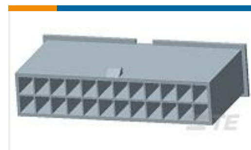
TE Part #1-1969612-2 12P FH PLUG VAL-U-LOK V0
