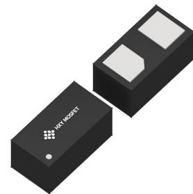
DFN0603-2L (DFN-2L(0.6x0.3))
