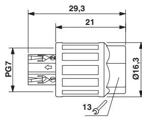
Dimensional drawing
