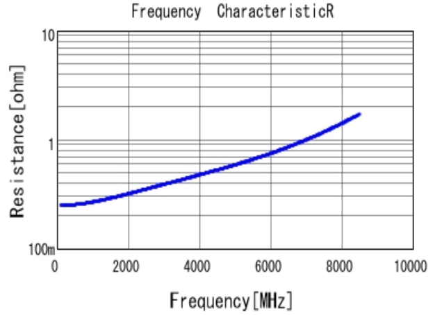
■ GRM0335C1H3R3BA01 R DC0V, 25degC
