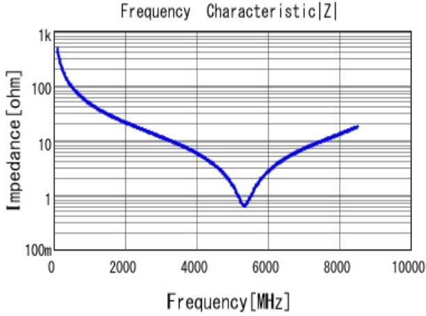
■ GRM0335C1H3R3BA01 |Z| DC0V, 25degC
