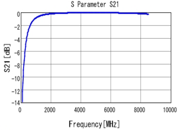
■ GRM0335C1H3R3BA01 S21 DCOV, 25degC
