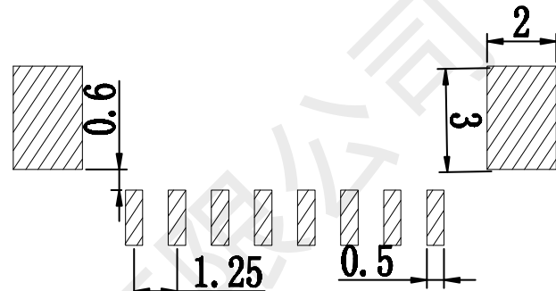
RECOMMENDED P. C. BOARD LAYOUT (TOP VIEW)
