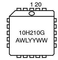
PLLC-20 FN SUFFIX CASE 775
