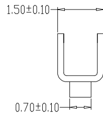
SEC:C-C
