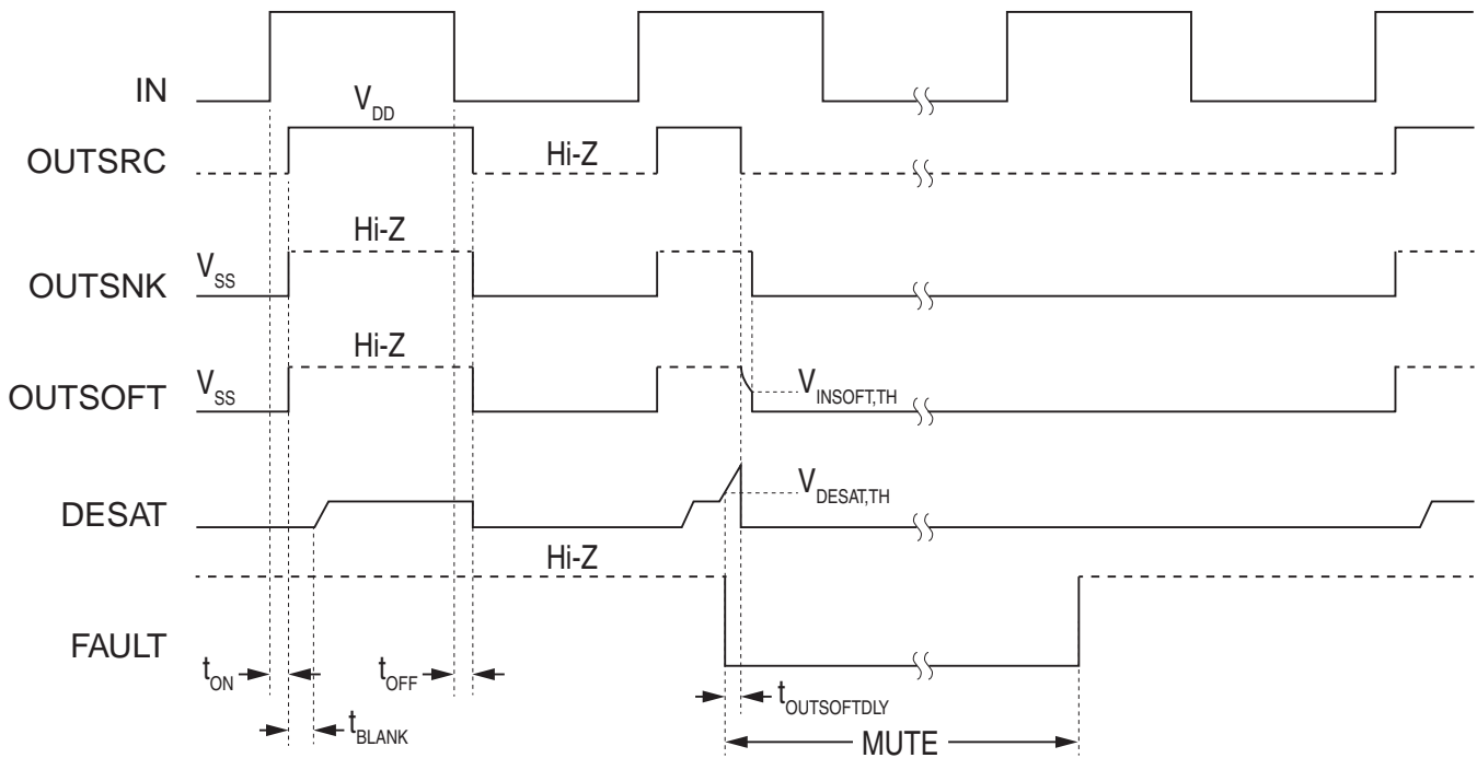
Figure 2. Timing Diagram
