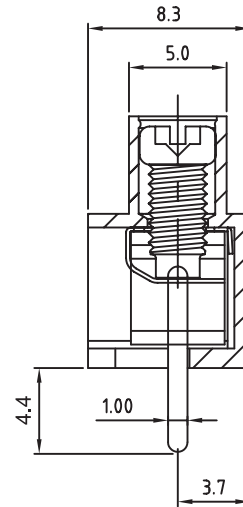
SECTION H-H
