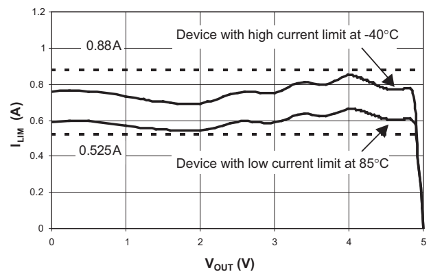
Figure 1: Output Current Using 10.5k\Omega .
