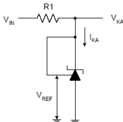
V_{REF} Test Circuit 5 for V_{KA} >
