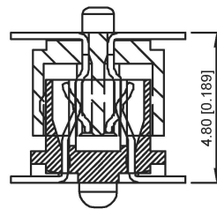
ASSEMBLY SCALE 2:1
