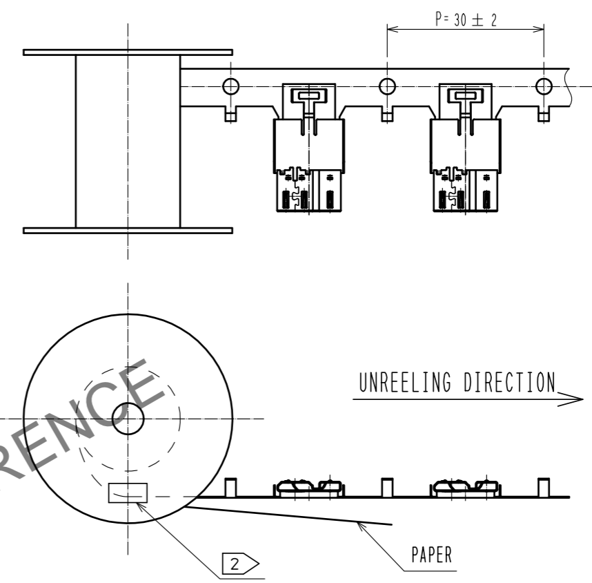
1 Fig-1 DRAWING FOR PACKING (FREE)
