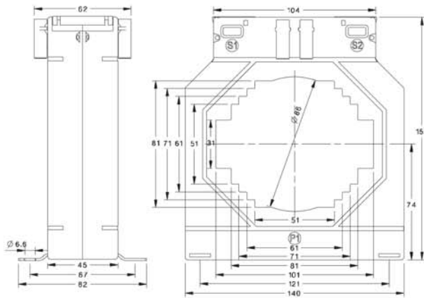
XMER 140-100H
