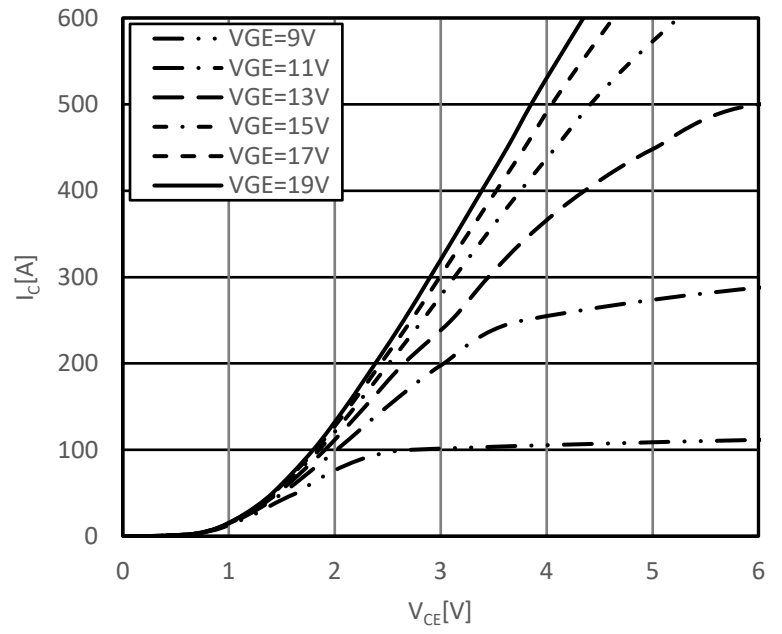
输出特性IGBT,逆变器 (典型) output characteristic IGBT,Inverter (typical) I_C=f(V_{CE}) T_{vj}=125^\circ C
