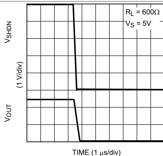
Figure 43. Turnoff Time
