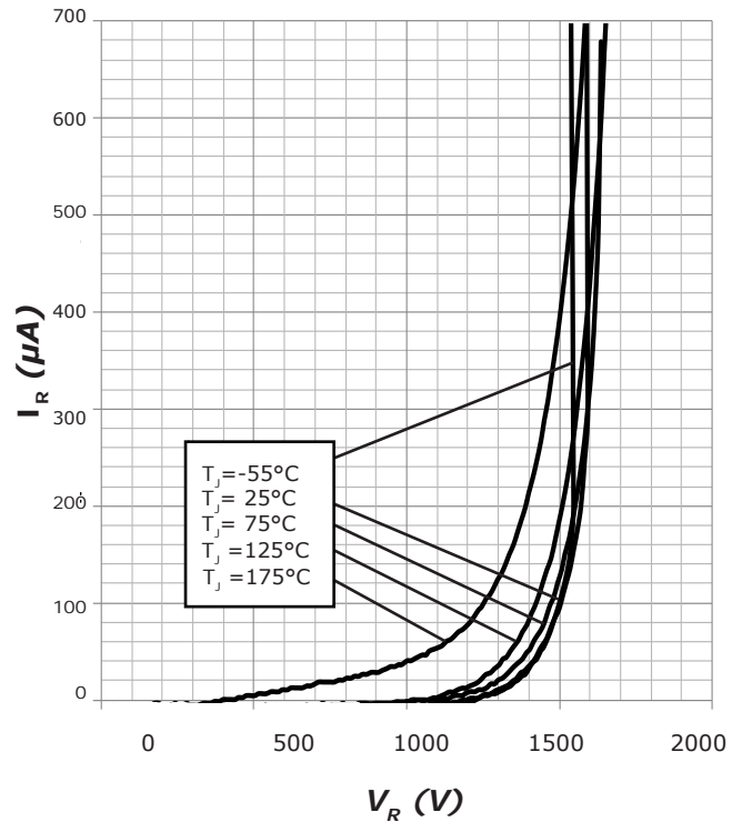
Figure 2. Reverse Characteristics
