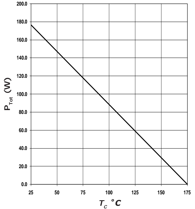
Figure 4. Power Derating
