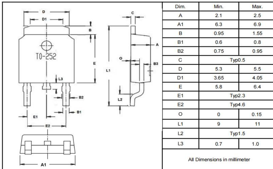
TO-252
