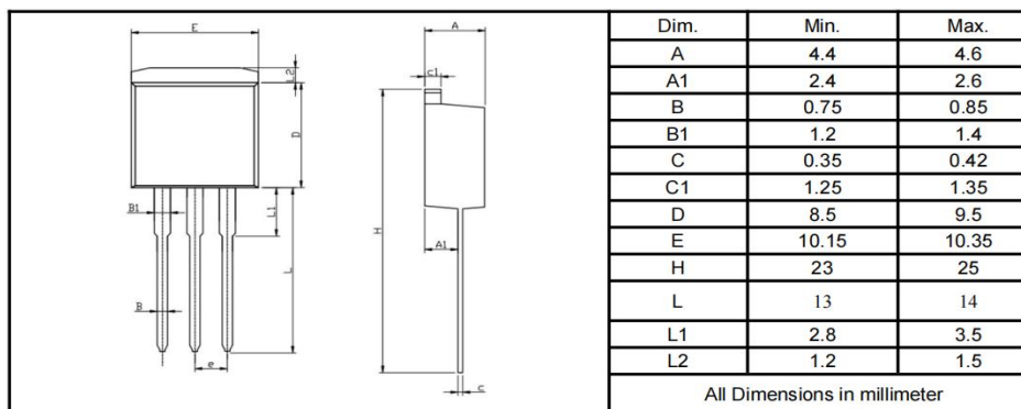
TO-262
