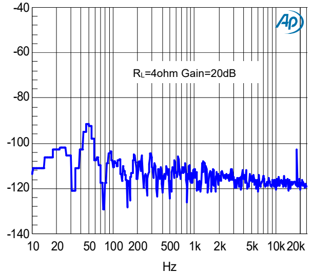
Noise Floor FFT
