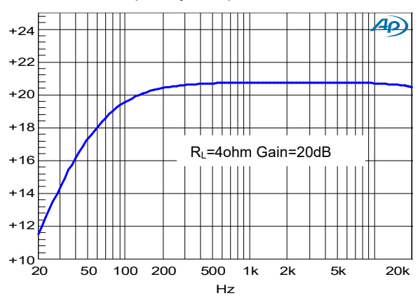
Frequency Response
