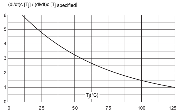
Relative variation of critical rate of decrease of main current versus (junction temperature (typical values)
