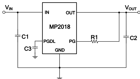
Figure 3: MP2018 Schematic
