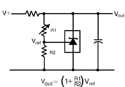
FIGURE 1. SHUNT REGULATOR
