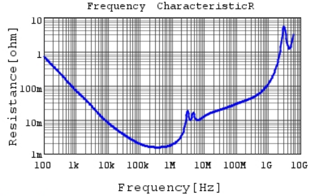
GCM32EC7YA106KA03 R DCOV, 25degC
