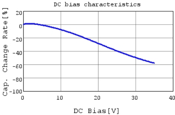
GCM32EC7YA106KA03 C-DC bias capchange, 25.0c
