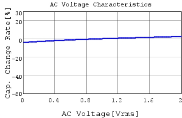
GCM32EC7YA106KA03 C-AC Voltage capchange, Dc
