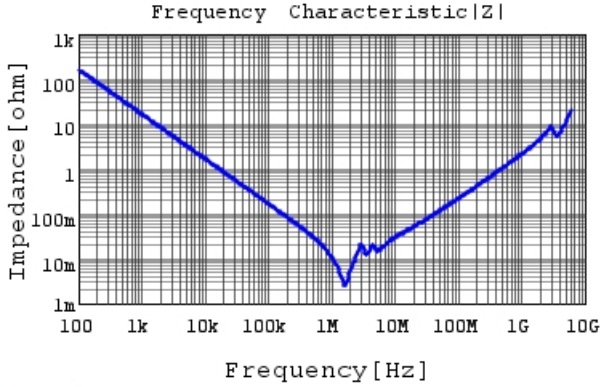
GCM32EC7YA106KA03 |Z| DCOV, 25degC
