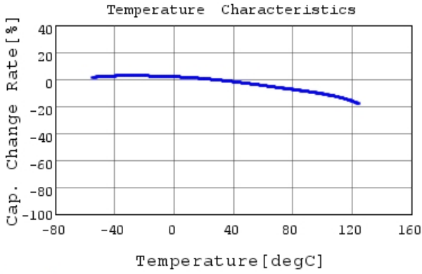
GCM32EC7YA106KA03 C-Temp. capchange, DC0.0V,
