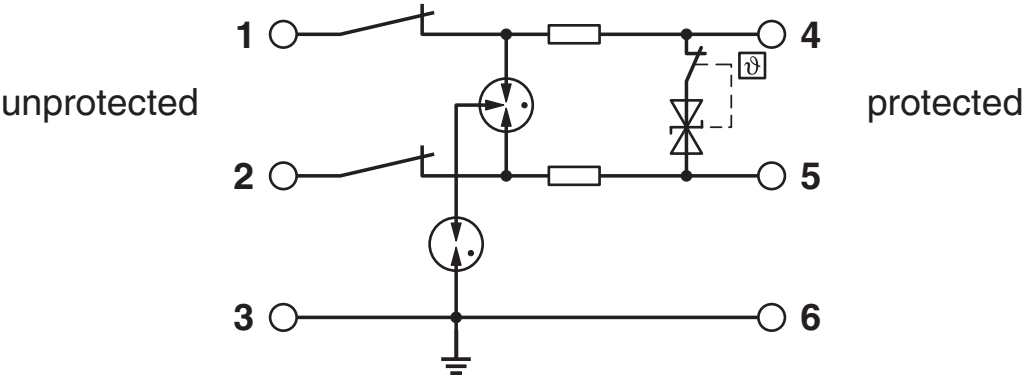
Circuit diagram
