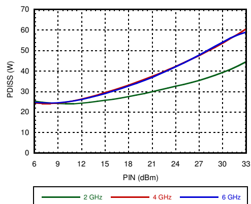
Power Dissipation vs. Pin
