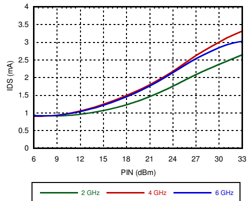
Drain Current vs. Pin
