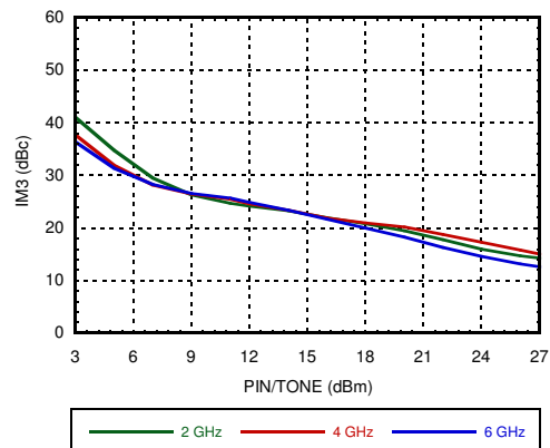
IM3 vs. Pin/Tone
