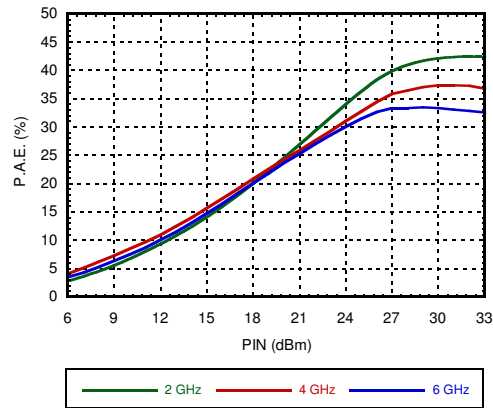
Power Added Efficiency vs. Pin
