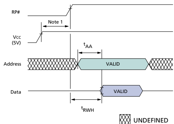
Figure 2: Power-Up/Reset Timing Diagram
