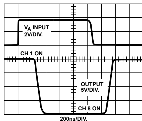
ACCESS TIME
